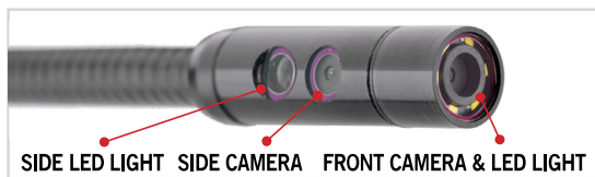
SIDE LED LIGHT SIDE CAMERA FRONT CAMERA & LED LIGHT
